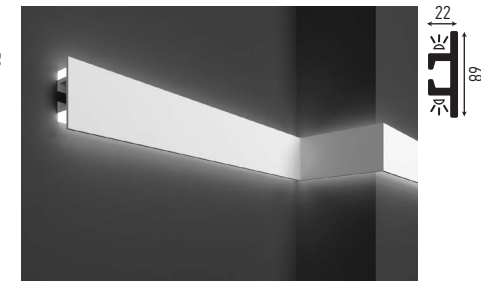
KH 907 68 x 22 mm
