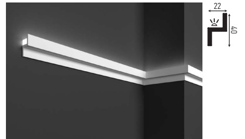
KH 902 40 x 22 mm
