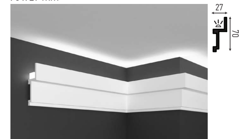
KH 915 70 x 27 mm
